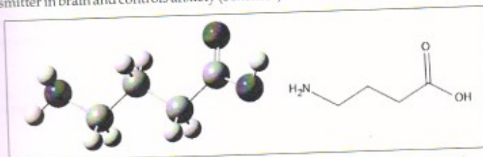
Scheme I- Structure of brain chemical GABA i.e. \gamma -Aminobutyric acid
